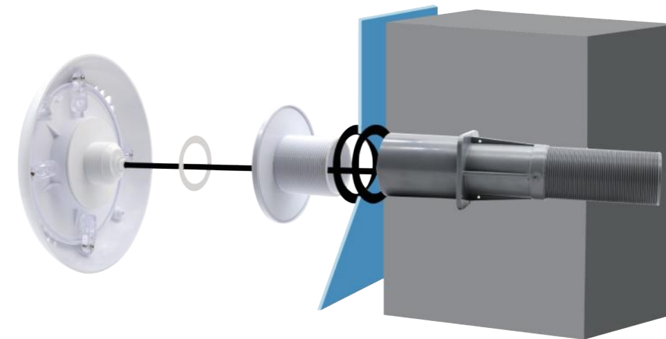
Concrete+Liner pool
